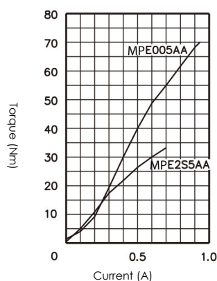
Standard torque chart
