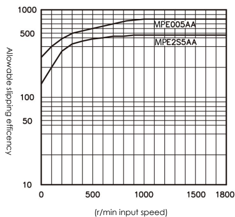
Allowable slipping efficiency chart
