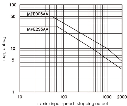
Allowable slipping torque chart
