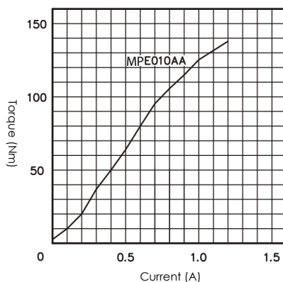
Allowable slipping torque chart
